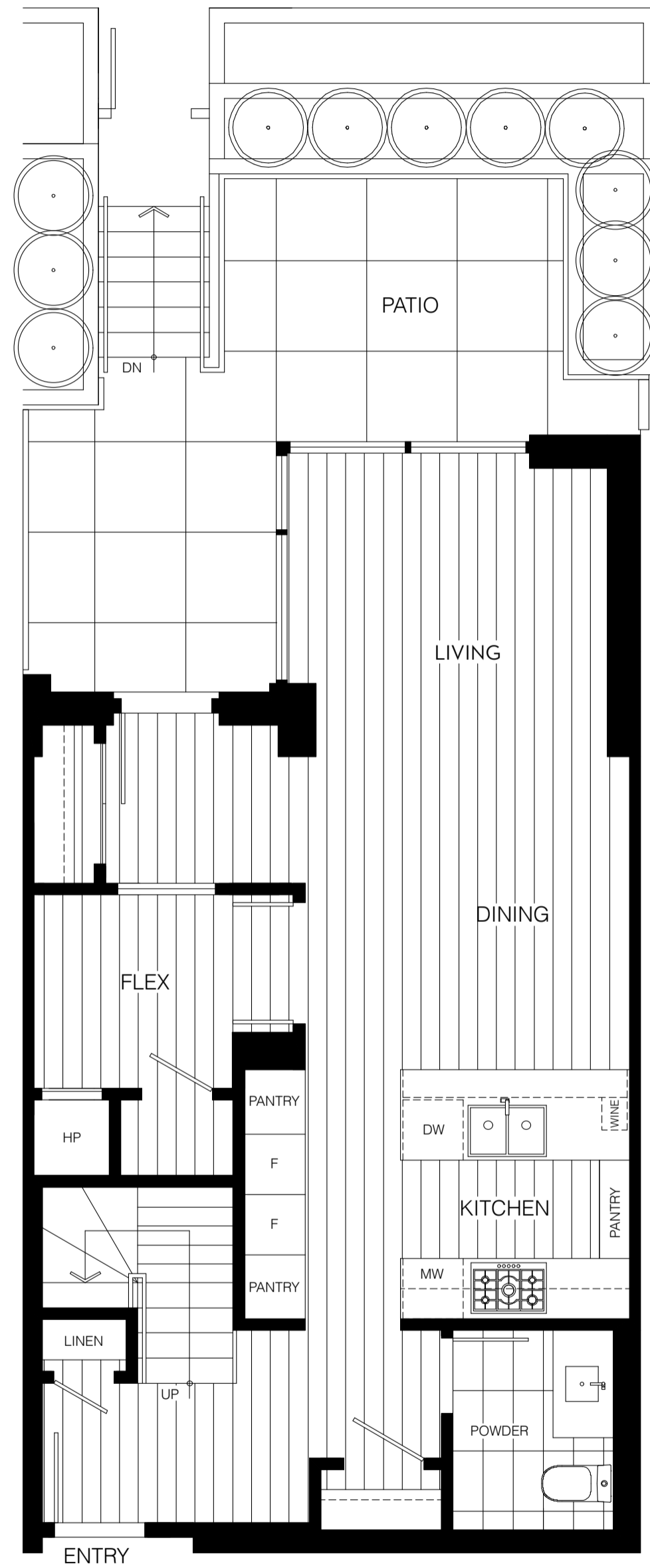
MAIN
